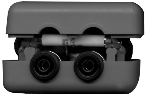
Fig.23 Fuse Location
