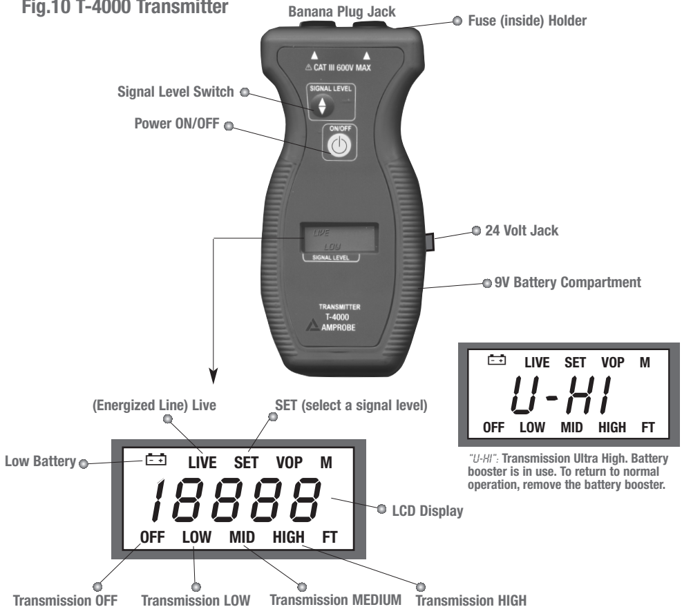
Fig.10 T-4000 Transmitter
