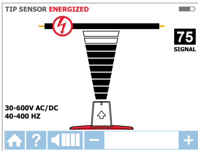
Figure 3.1i Receiver showing signal detected in Energized TIP SENSOR mode
